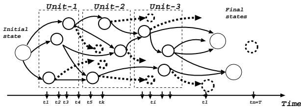
Figure 2: Illustration of the execution paths with multiple PRUs
